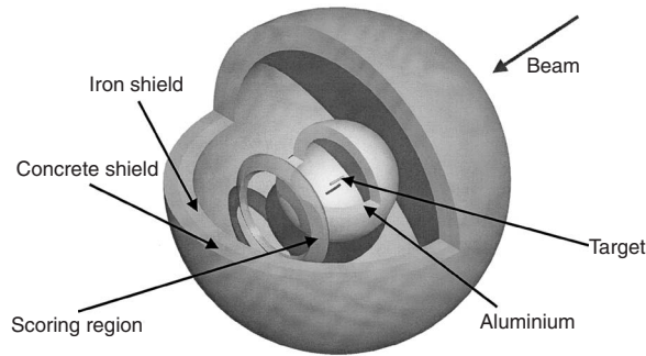
Figure 8. Simplified spherical geometry used in the preliminary calculations for the upgrade of the CERF facility to reproduce the radiation field in a space vessel.
