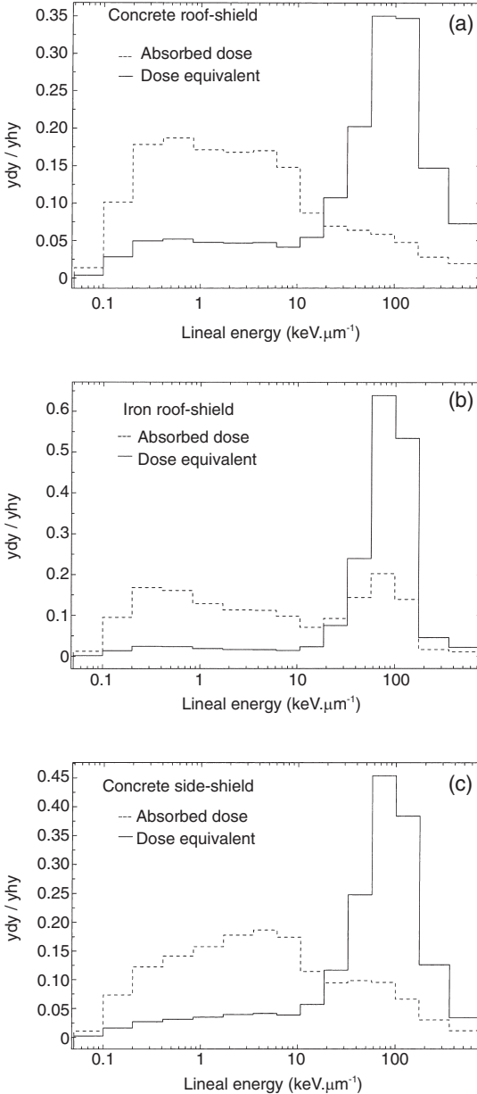
Figure 5. Distribution of absorbed dose, d(y) , and dose equivalent, h(y) , in lineal energy y , measured with the HANDI TEPC on the concrete roof-shield (a), on the iron roof-shield (b) and on the 80 cm thick concrete side-shield (c).
