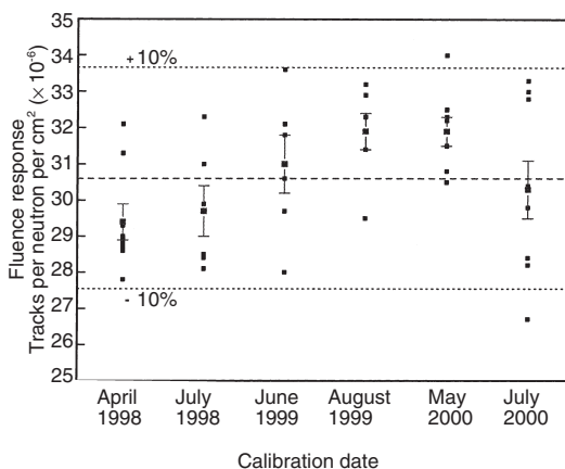
Figure 7. Calibration measurements of the NRPB passive survey meter, PADC neutron detectors at CERF (April 1998 to July 2000) (12) . Small symbols, individual sheet results. Large symbol, mean for that measurement \pm SEM. (---) overall mean = 30.6 \pm 0.3 (SEM).
