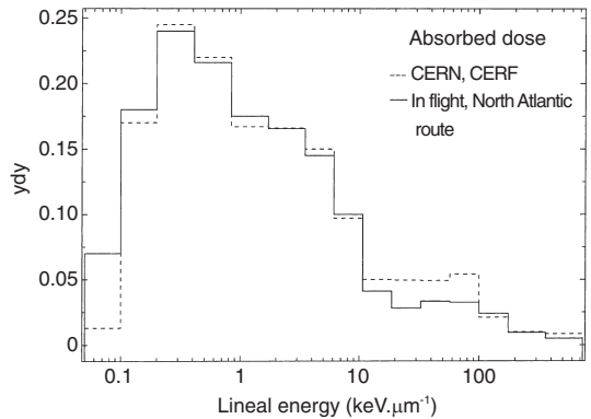
Figure 6. Distribution of absorbed dose, d(y) , in lineal energy y , on the concrete roof-shield of CERF and at flight altitude on a north Atlantic route (37) , normalised to the same total dose.
