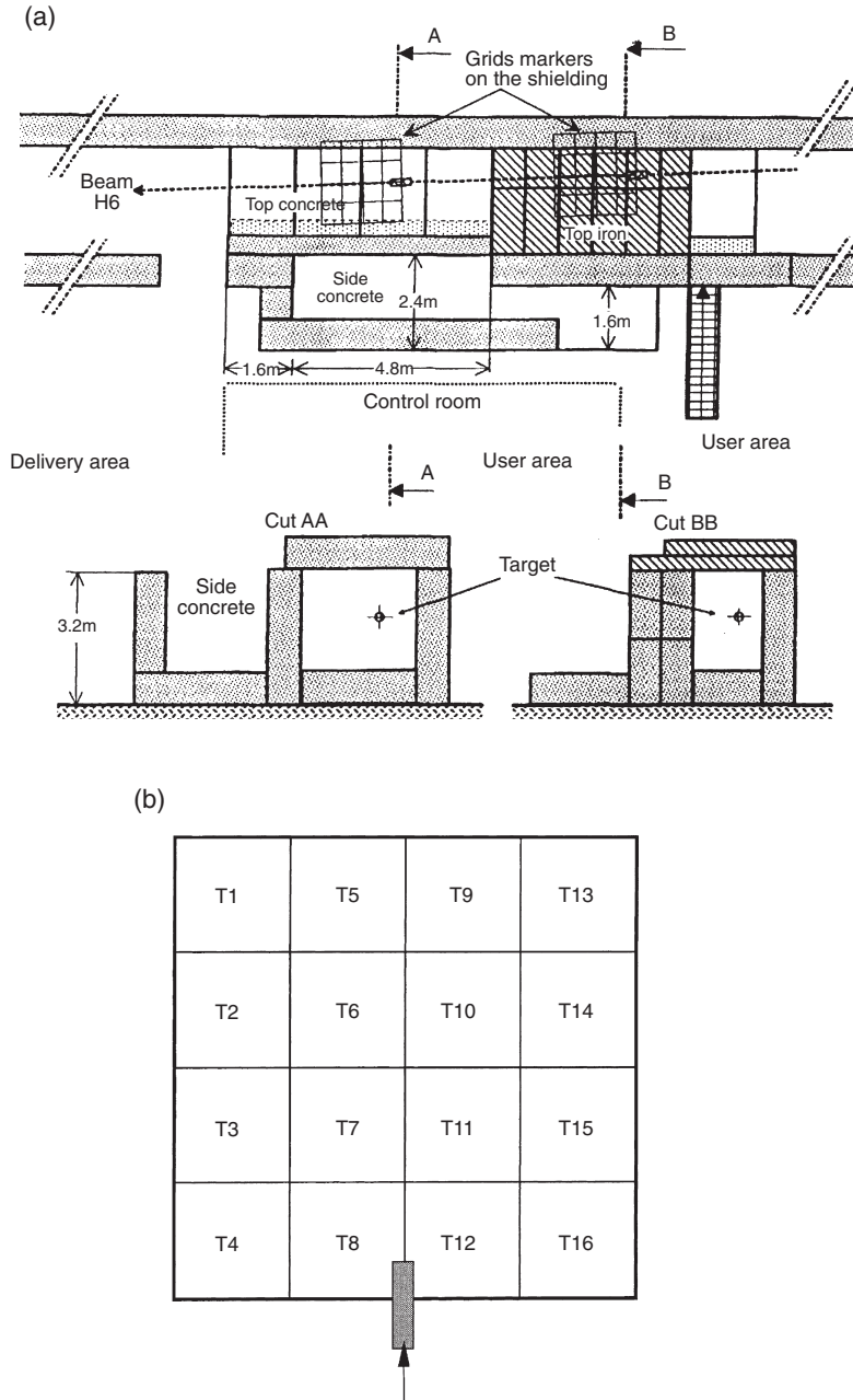
Figure 3. (a) Plan and sectional views of the CERF facility. (b) The reference grid with the 16 exposure locations used on the concrete and iron roof-shields.
