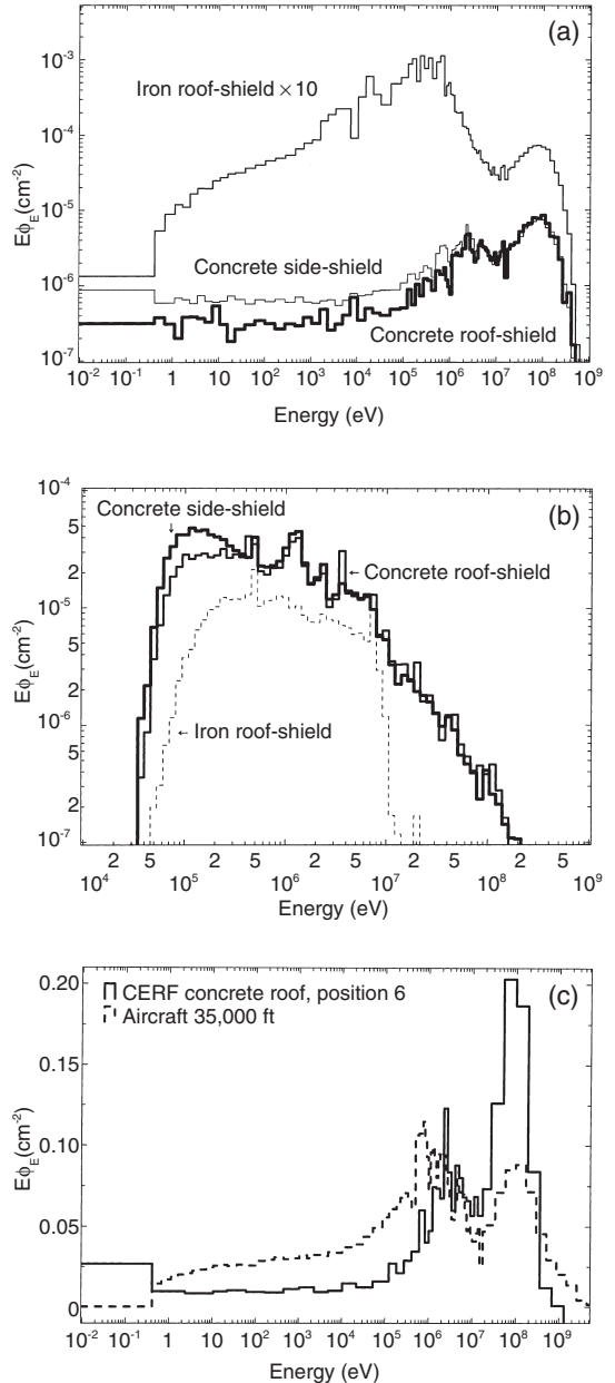
Figure 4. Neutron (a) and photon (b) spectral fluences on the concrete roof-shield, on the iron roof-shield and on the 80 cm thick concrete side-shield (neutrons or photons per primary beam particle incident on the copper target). (c) Comparison of the CERF neutron spectrum on the concrete roof-shield (position 6 on the grid of Figure 3(b)) with the neutron spectrum at an altitude of 10.6 km (35,000 feet) as calculated by Heinrich et al. (26) . The total fluence is normalised to unity.
