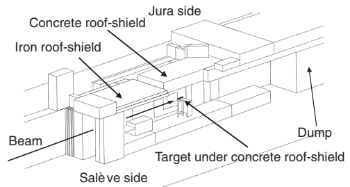
Figure 2. Axonometric view of the CERF facility in the North Experimental Hall on the Prévessin site of CERN as modelled in FLUKA. The side shielding on the Salève side is removed to show the inside of the irradiation cave with the copper target set-up.
