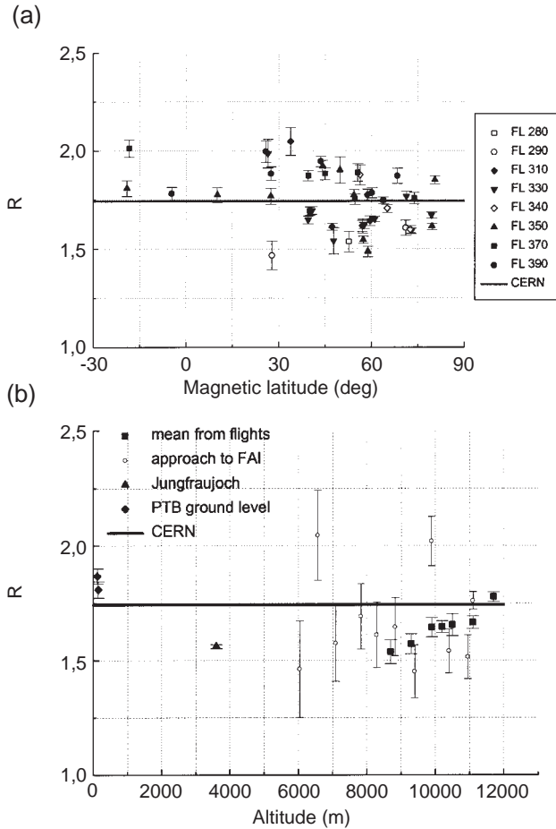
Figure 2. (a) Ratio, R , of neutron dose equivalent readings (lead-modified A&B rem counter divided by the standard A&B rem counter) as a function of the magnetic latitude. The data points are the results from in-flight measurements averaged during the time of continuously flying at the flight level altitude, FL, indicated by the symbol (FL is the unit for the air pressure altitude commonly used in aviation; for standard atmospheric conditions the conversion factor is: 30.48 m per FL). The horizontal line represents R measured for the CERN concrete field. (b) Mean R shown in Figure 2(a) plotted as a function of altitude. The PTB measurements were performed in a wooden hut (altitude: 120 m) and on top of a tower 30 m high at a measuring place surrounded by low mass walls (altitude: 150 m). The Jungfrauoch measurements were performed in the astronomical observatory on top of the Alpine Research Facility (altitude 3600 m). The measurements during the approach to FAI were performed by descending at a slow, constant rate.
