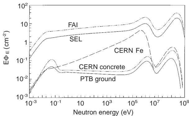
Figure 4. Comparison of the neutron energy distribution of fluences from in-flight measurements (FAI = position in the vicinity of Fairbanks, Alaska, USA, altitude FL = 330 (10,058 m); SEL = position Seoul, Korea, altitude FL = 330 (10,058 m)) CERN calibration field measurements behind shieldings of concrete (80 cm) and iron (40 cm) and PTB ground level measurement ( E denotes the neutron energy and \Phi_E = d\Phi/dE the energy distribution of fluence).
