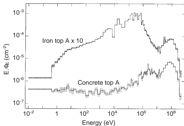
Figure 1. Neutron energy distribution of fluence for the CERN calibration fields behind shieldings of 80 cm of concrete and 40 cm of iron, respectively, calculated with the Monte Carlo code FLUKA ( E denotes the neutron energy and \Phi_E = d\Phi/dE the energy distribution of fluence).
